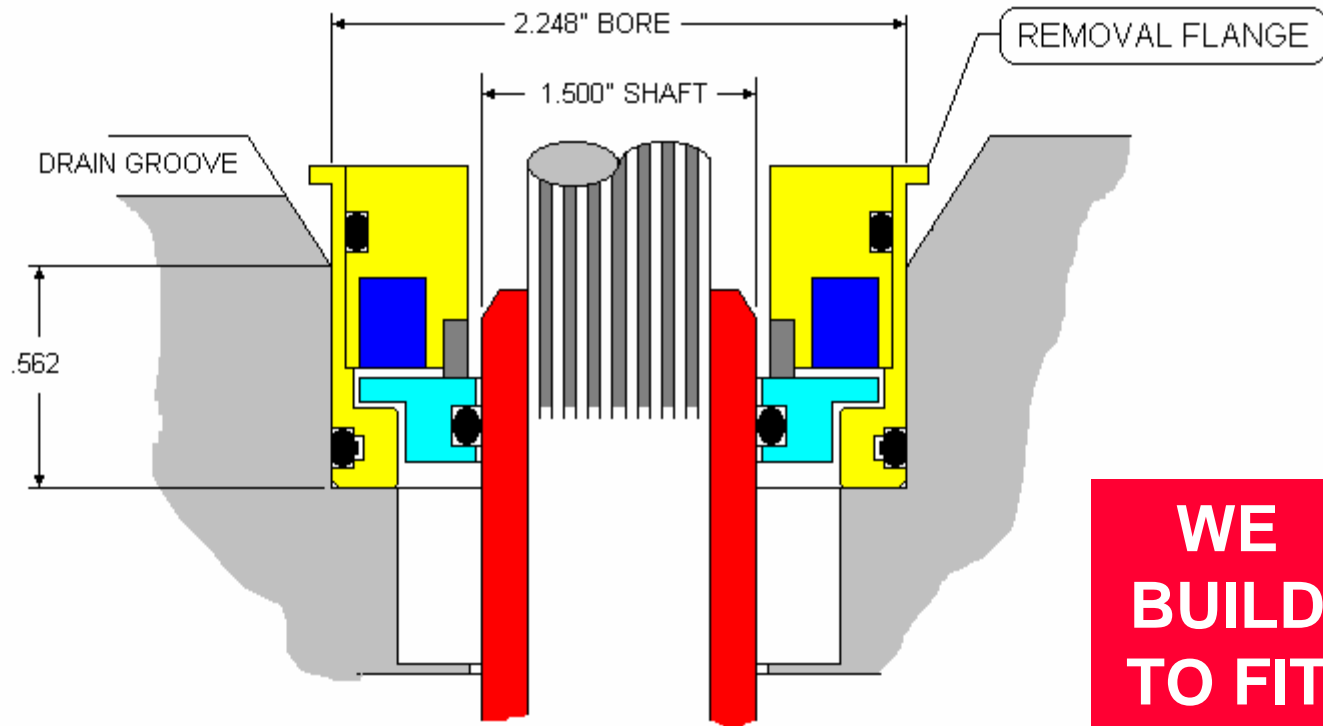
ISOMAG MAGNUM-S BEARING SEAL INSTALLED IN UPPER GEAR BOX OF SUNDYNE PUMP 1.500" SHAFT DIA.
